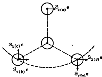
FIG. 5.—Diagram of \text{CO}_3^- group. The electric vector is parallel to the line joining the two oxygens. (Bragg.)
